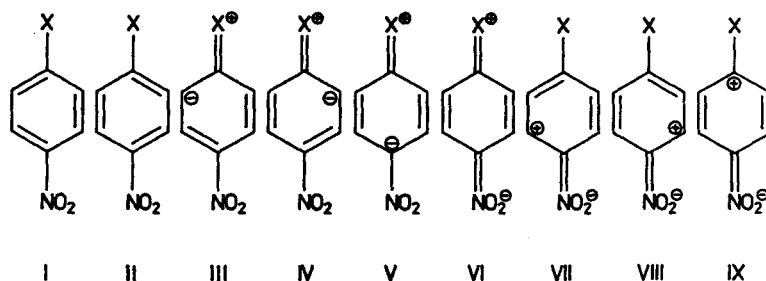
Figure 2. Canonical structures describing para -substituted nitrobenzenes
