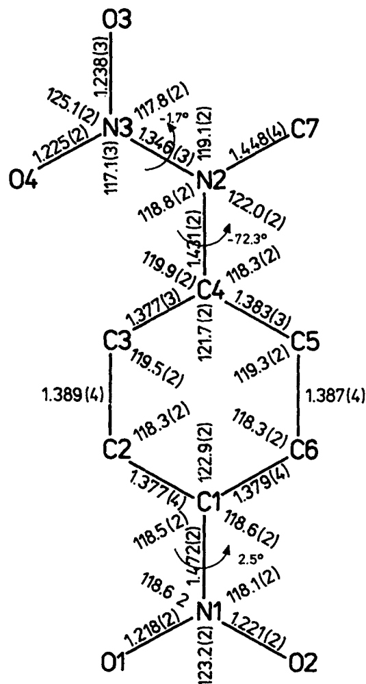
Figure 1. Values of bond lengths, bond angles and dihedral angles between the best ring planes
